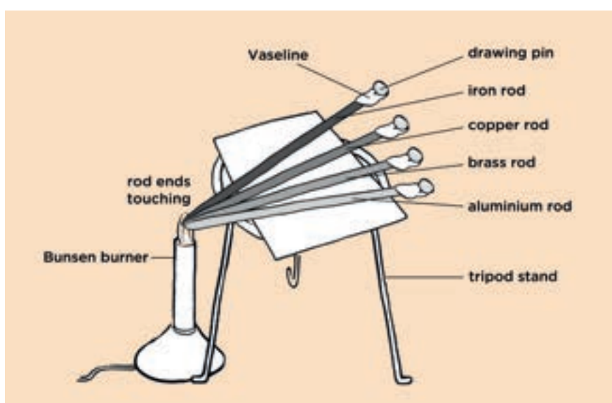
Fig. 2.3: Testing the conductivity of metals
