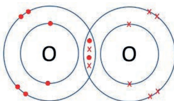
Fig. 2.11: Formation of molecule of Oxygen Gas ( \text{O}_2 )
