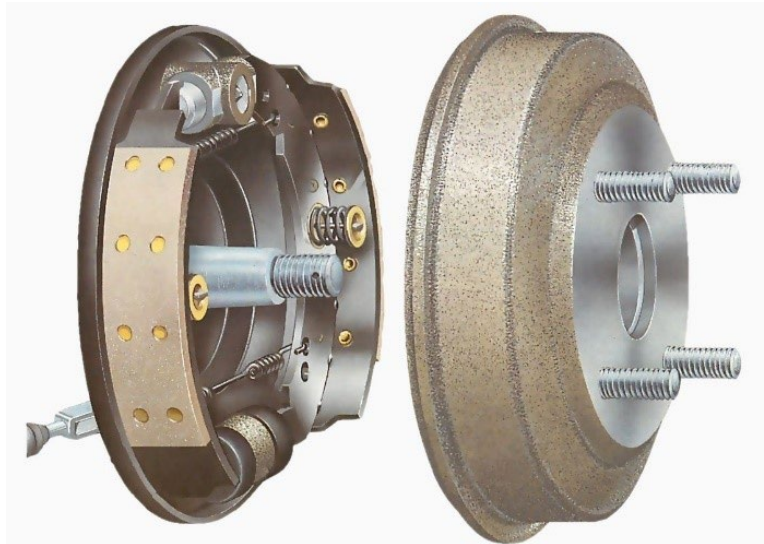
Fig. 5.2.9: Brake drum and shoes assembly
