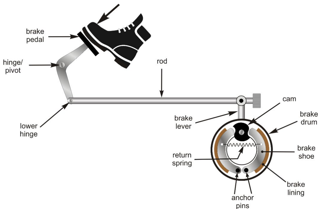
Fig. 5.1.1: A mechanical brake
