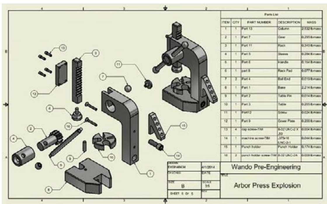
Fig. 8.13: A Picture of components of an Arbor Press
