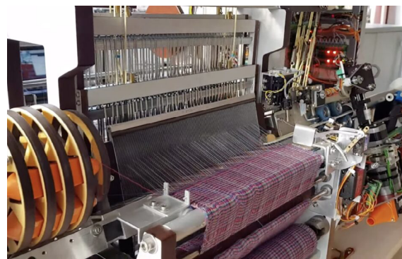
Fig. 6.6. Weaving Machine
