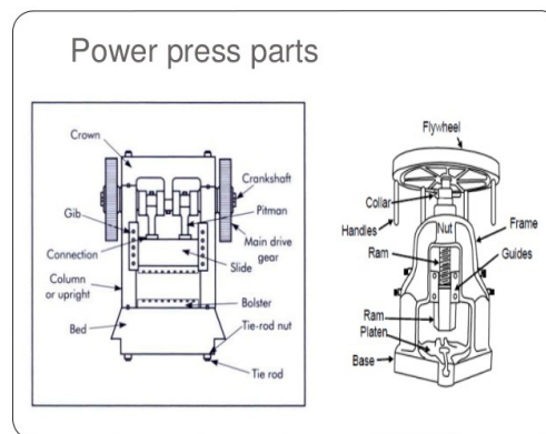
Figure. 5.20.5: Press working Terminologies
