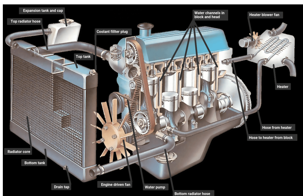
Figure 1.3.1: Parts of water-cooling system
