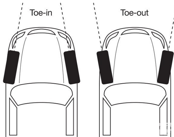
Figure. 4.15.12: Toe-in and toe-out.
