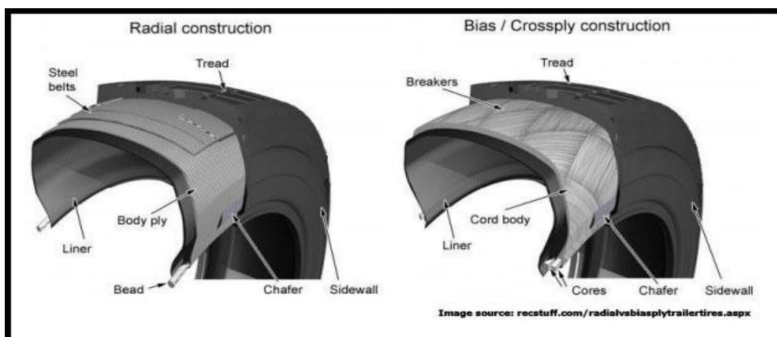
Figure 6.23.10: Radial-ply and cross-ply tyre construction
