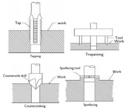
Figure 1.4.4: Applications of a twist drill
