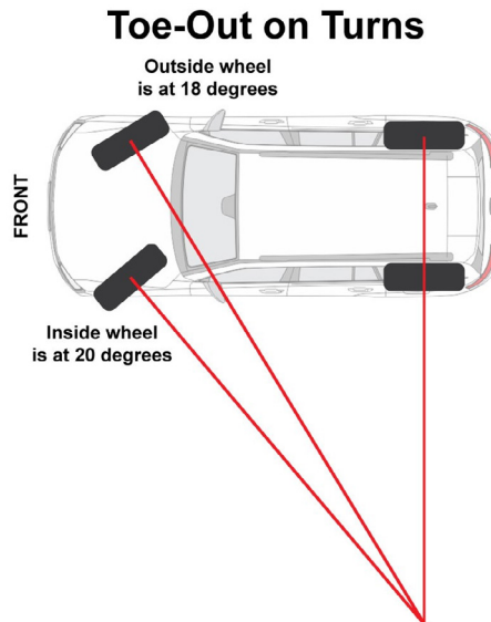
Figure. 4.15.14: Toe-out on turns
