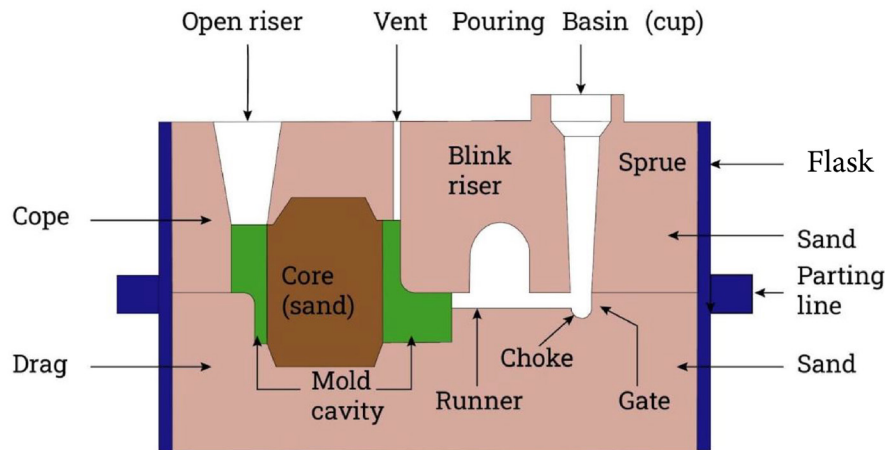
Figure. 3.12.3: Parts of the sand-casting mould
