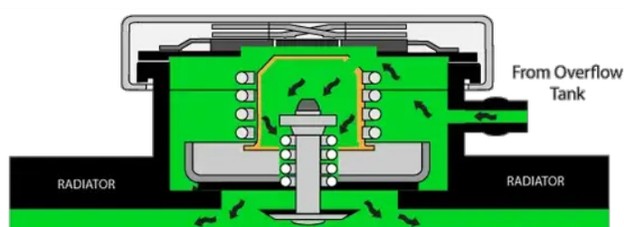
Figure. 2.5.5: Radiator pressure cap (coolant contraction stage)
