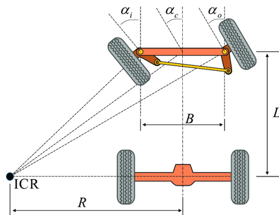
Figure. 4.15.13: Ackermann steering geometry
