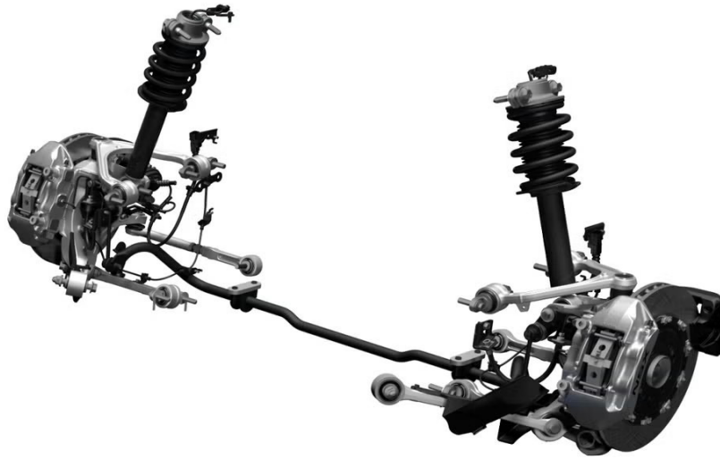
Figure 6.21.13: The double wishbone multi-link combination
