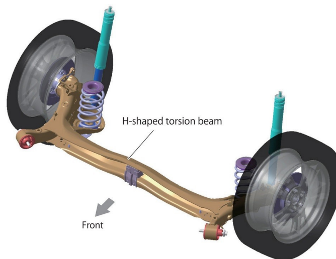
Figure. 5.17.5: Dependent/axle beam suspension system
