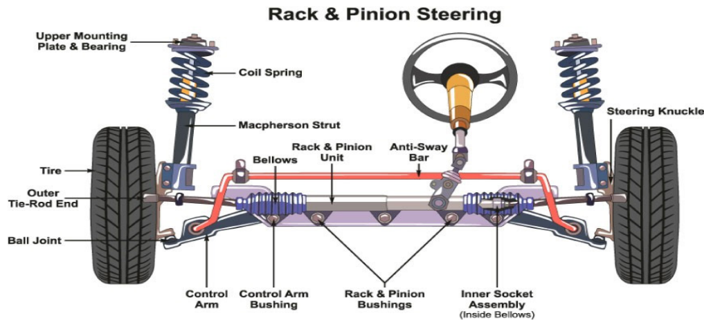
Figure. 4.15.1: The automobile steering system (Source: thors.com)
