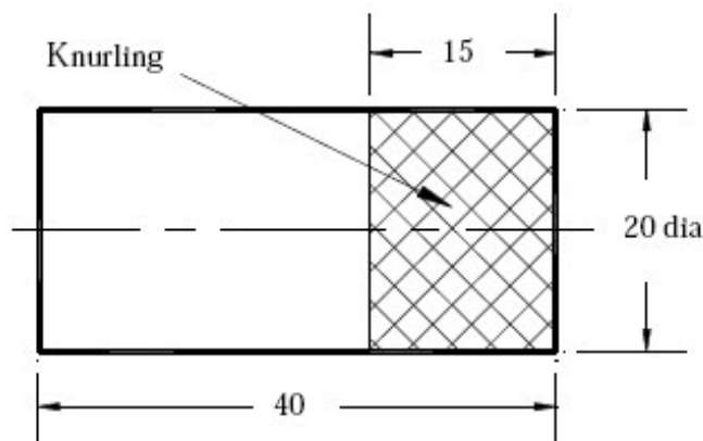
Figure. 3.10.4: Component to be produced
