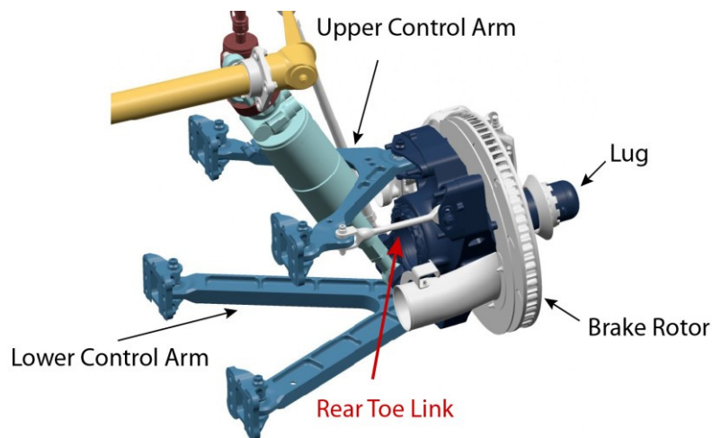
Figure 6.21.11: Toe-control link suspension.
