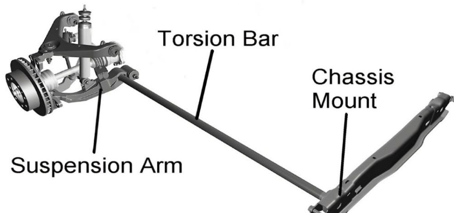
Figure. 5.19.7: Torsion bar assembly.
