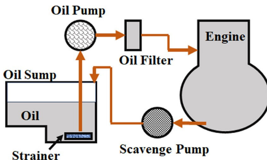
Figure. 3.9.3: Dry sump lubrication system
