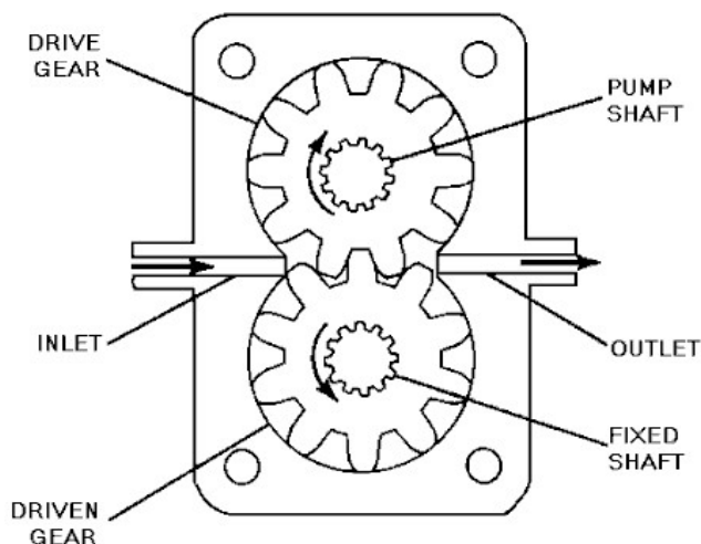
Figure. 3.9.4: Gear-type oil pump
