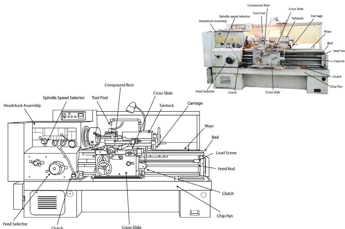
Figure. 2.6.1: Main parts of the lathe machine
