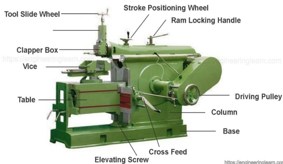
Figure. 2.6.5: Standard Shaper
