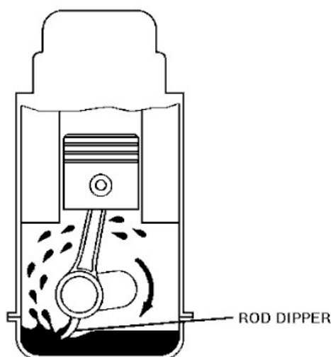
Figure. 3.9.1: Splash lubrication system
