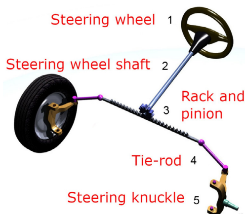
Figure 4.15.5: Components of the manual steering system
