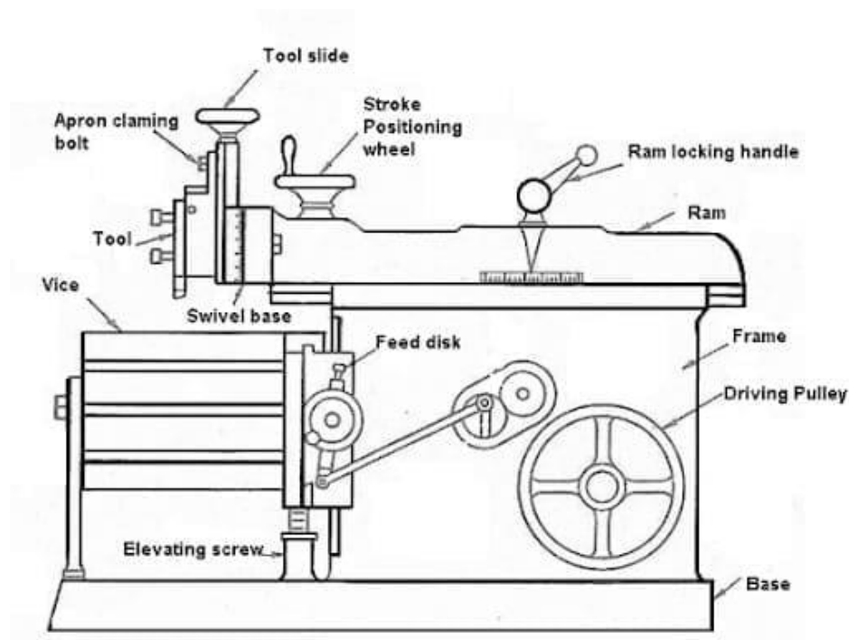
Figure. 2.6.4: Principal parts of a shaper
