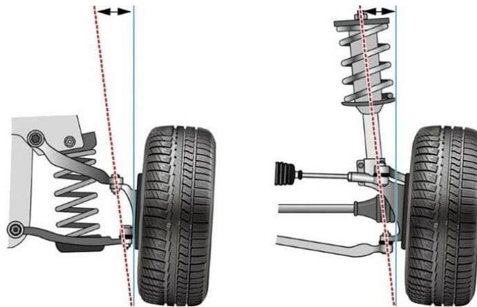
Figure. 4.15.10: Steering axis inclination and kingpin inclination
