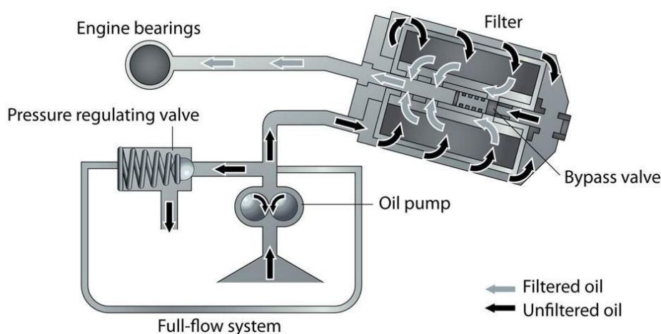
Figure. 3.9.8: Full-flow filter system
