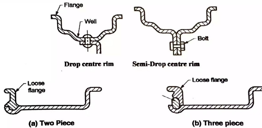
Figure 6.23.6: Flat-base rims
