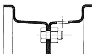
Figure 6.23.8: A divided rim
