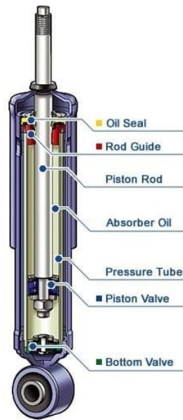
Figure. 5.17.2: A damper.
