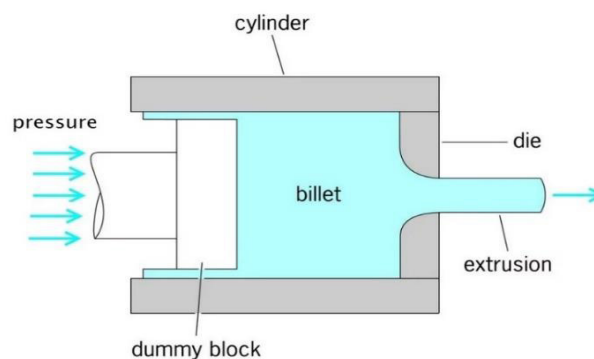
Figure. 4.16.9: Extrusion
