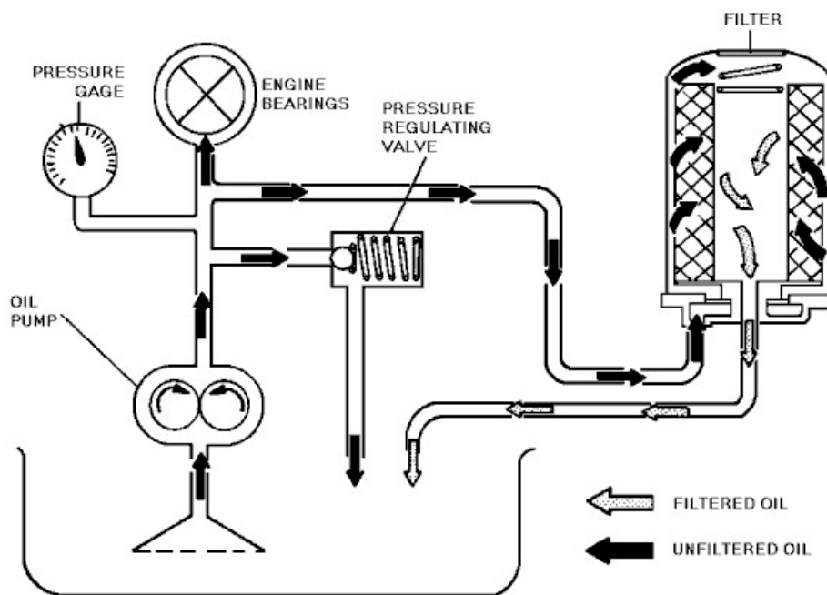
Figure. 3.9.9: Bypass filter system
