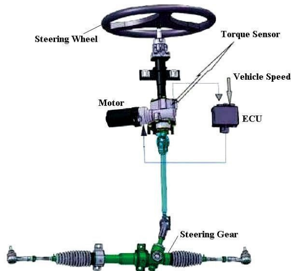
Figure. 4.15.3: Electric power steering.
