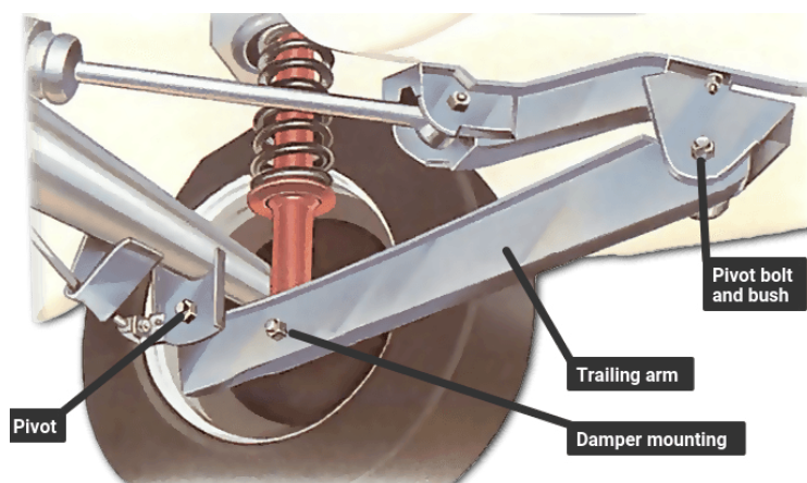
Figure 6.21.5: Trailing arm linkage
