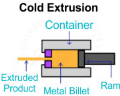
Figure 4.16.12: Cold Extrusion
