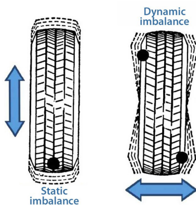
Figure 6.23.13: Static and dynamic imbalance
