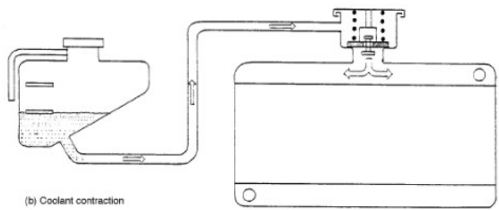
b. Coolant contraction stage Figure. 2.5.6: Sealed cooling systems
