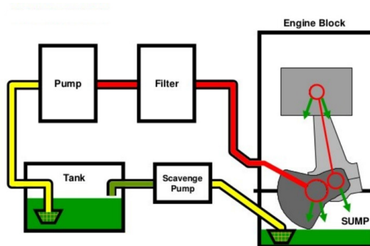
Figure. 2.7.4: Dry sump lubrication system.
