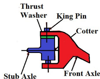
Figure. 4.13.5: Elliot stub axle
