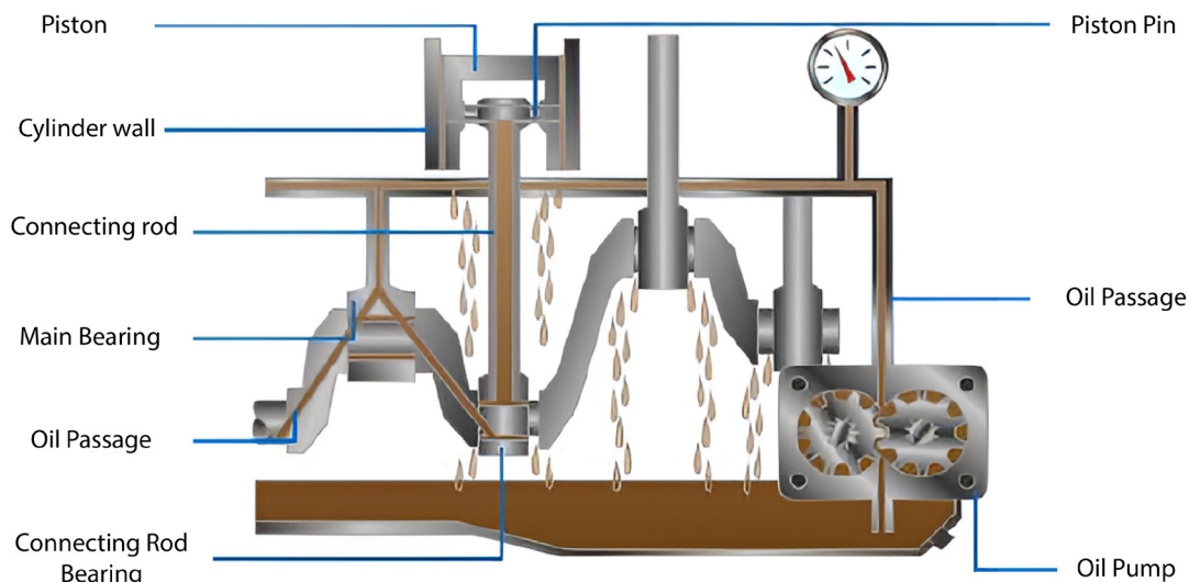
Figure. 3.9.2: Pressure lubrication system
