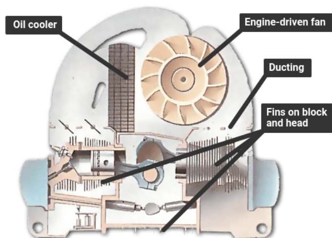
Figure 1.1.1: Features of an air-cooled engine
