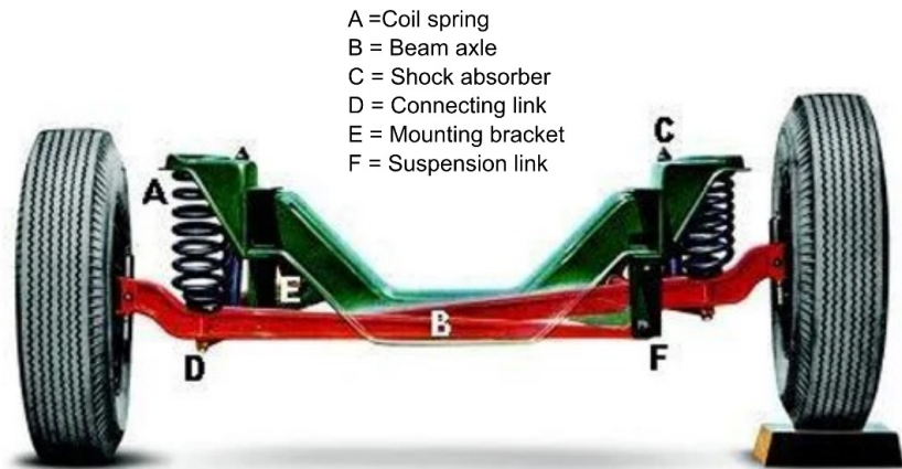
Figure 6.21.1: Dependent beam axle suspension system
