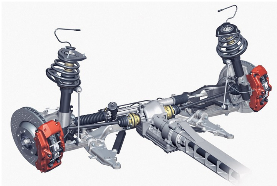
Figure. 6.21.10: MacPherson strut suspension
