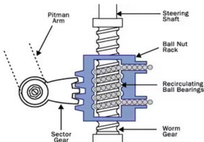
Figure. 4.15.7: A recirculating ball gearbox mechanism
