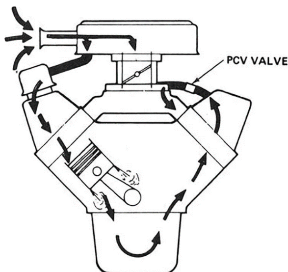
Figure. 3.11.4: A positive crankcase ventilation
