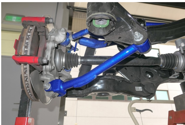
Figure 6.21.12: Trailing arm suspension
