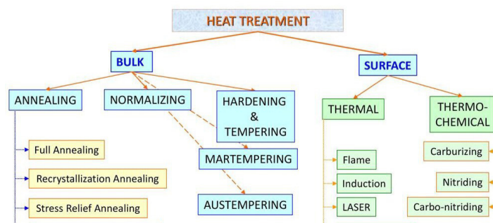
Figure 1.2.1: Flow chart of Heat Treatment Process.
