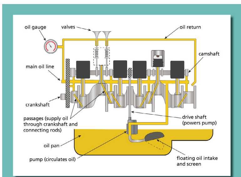
Figure. 2.7.1: Layout of the engine lubrication system
