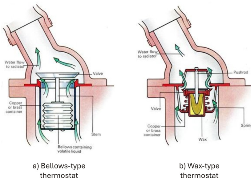
Figure. 2.5.1: Bellows-type and wax-type thermostats (Source: uk.pinterest.com)
