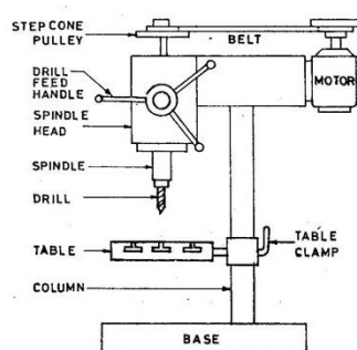
Figure 1.4.6: Parts of a drilling machine
