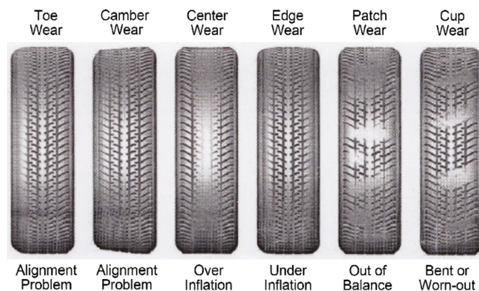
Figure 6.23.12: Uneven or abnormal tyre wear (Source: www.researchgate.net )
