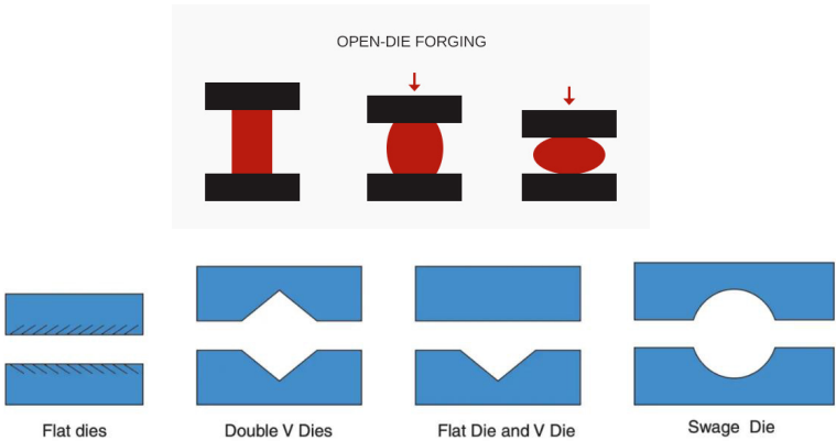
Figure. 4.16.4: Open die forging
