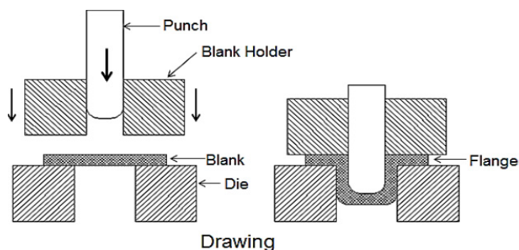
Figure. 5.20.1: Drawing
