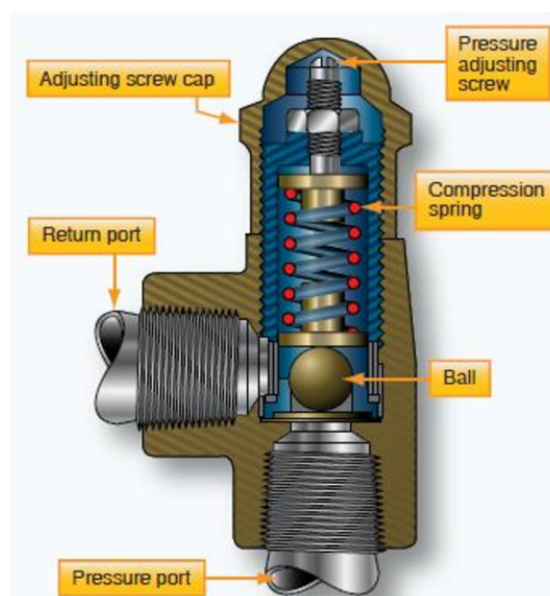
Figure. 3.9.7: Pressure relief valve
