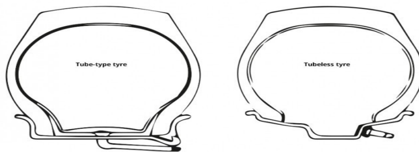
Figure 6.23.9: Tubed and tubeless tyre designs
