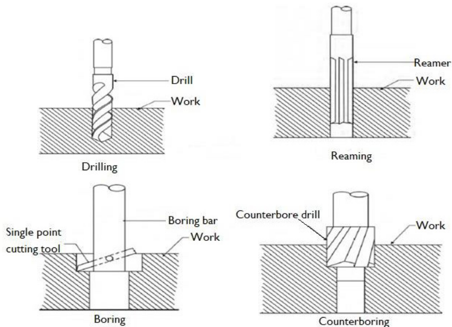
Figure 1.4.3: Applications of a twist drill
