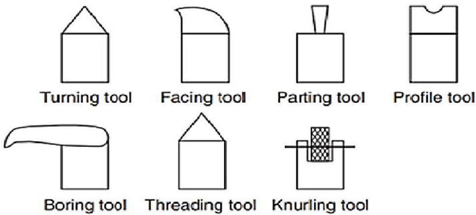
Figure. 3.10.3: Right-hand lathe tools
