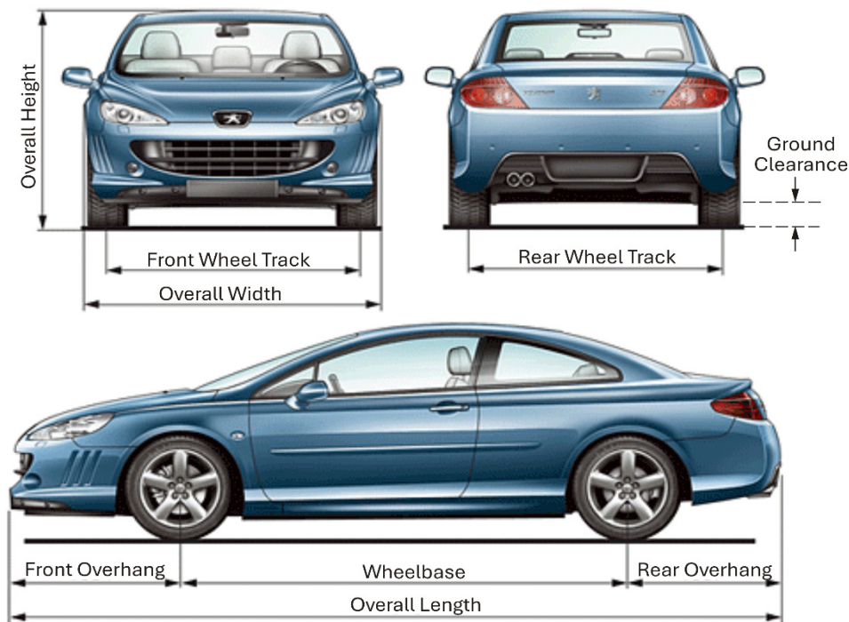
Figure. 4.13.9: Vehicle dimensions
