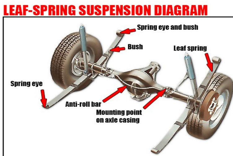
Figure. 5.19.1: Leaf spring in suspension
