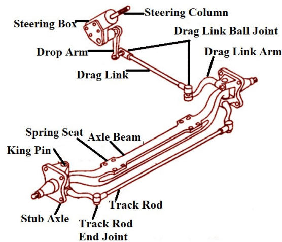
Figure. 4.13.2: An ‘I’ section dead front axle
