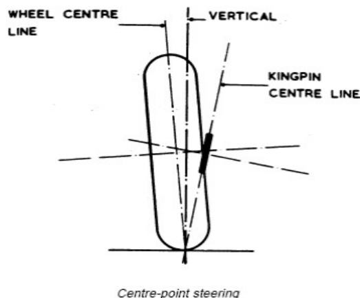
Figure. 4.15.11: Centre point steering
