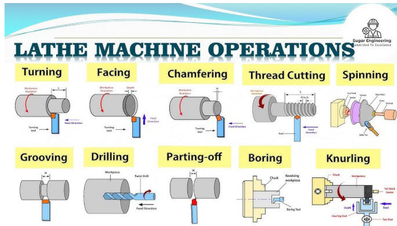
Figure. 2.6.3: Lathe operations
