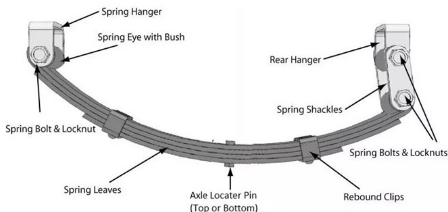
Figure. 5.19.2: Parts of a leaf spring
