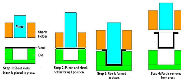
Figure. 5.20.4: Sheet metal deep drawing process
