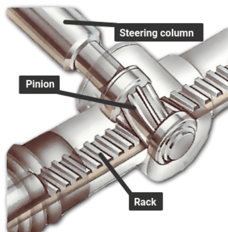
Figure. 4.15.6: A rack and pinion steering mechanism
