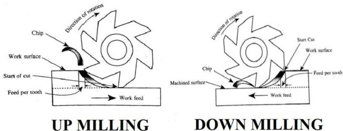
Figure. 2.8.2: Up milling and down milling operations
