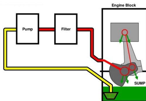
Figure. 2.7.3: Wet sump lubrication system
