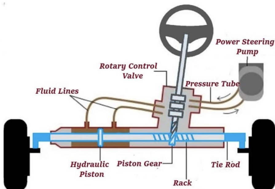
Figure. 4.15.4: Hydraulic power-assisted steering
