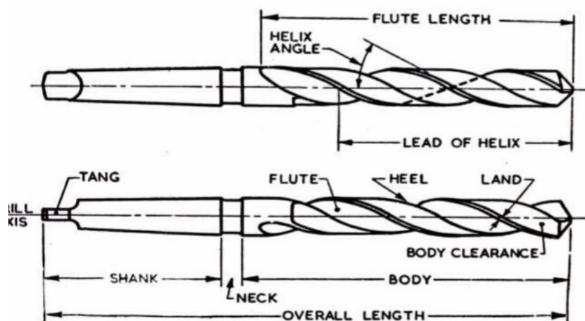
Figure 1.4.1: Parts of a twist drill.
