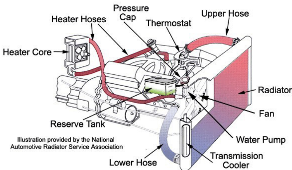
Figure 1.3.8: Pump-assisted water-cooling system
