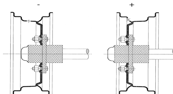
Figure 6.23.5: A well-base rim
