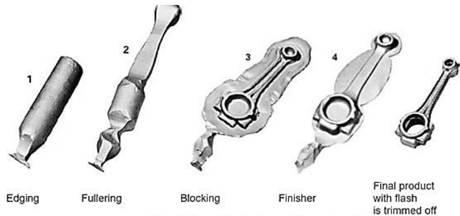
Figure. 4.16.1 Steps to follow in forging of a Connecting Rod
