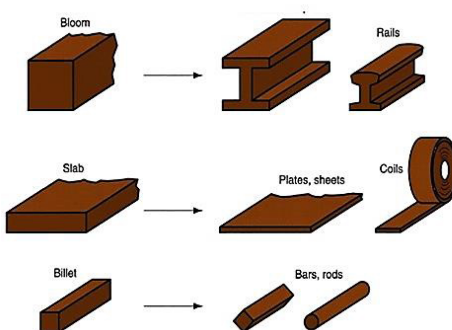
Figure. 4.16.8: Some of the steel products made in a rolling mill.
