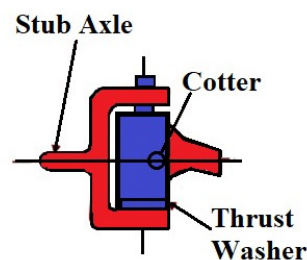
Figure. 4.13.6: Reversed Elliot stub axle
