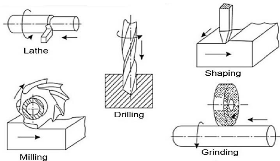
Figure. 3.10.2: Various machining processes with the various relative motions
