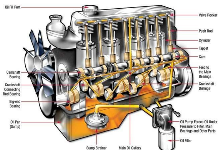
Figure. 2.7.2: Oil distribution channels in the engine.
