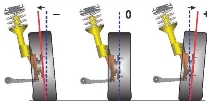
Figure. 4.15.9: Camber angles
