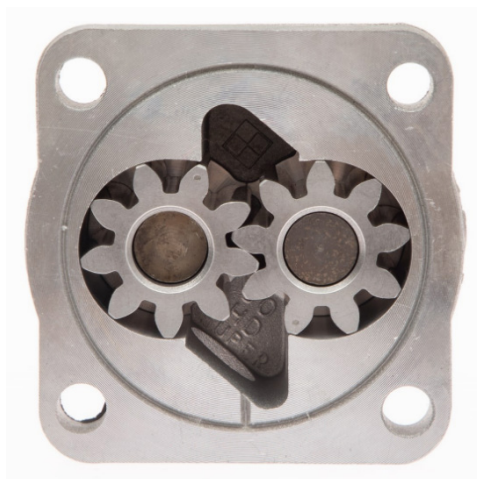
Figure. 2.7.7: Gear-type oil pump
