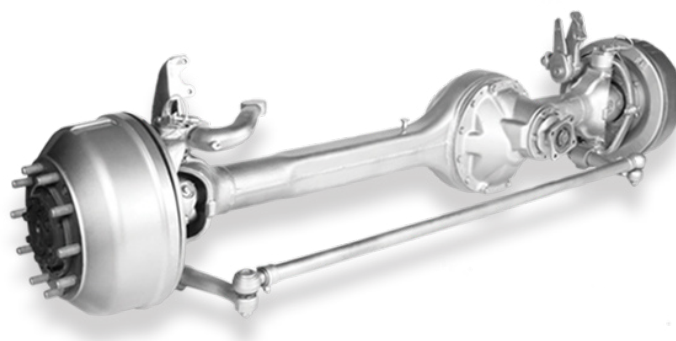
Figure. 4.13.3: A front live axle
