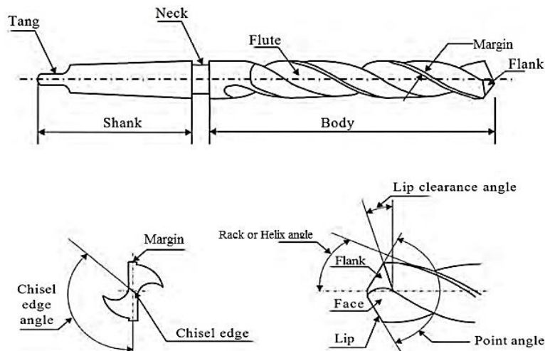
Figure 1.4.2: Parts of a twist drill
