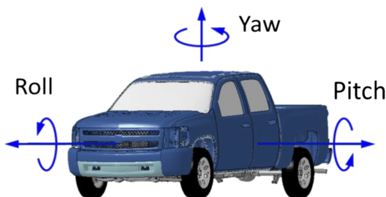
Figure. 5.17.7: Various suspension movements in vehicles
