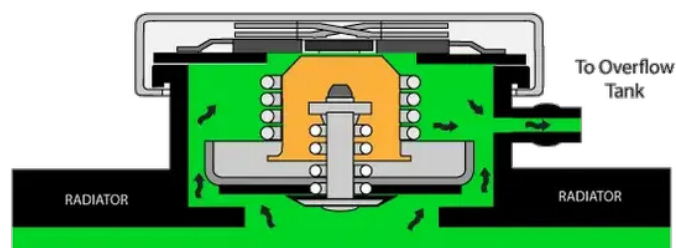
Figure. 2.5.4: Radiator pressure cap (coolant expansion stage)
