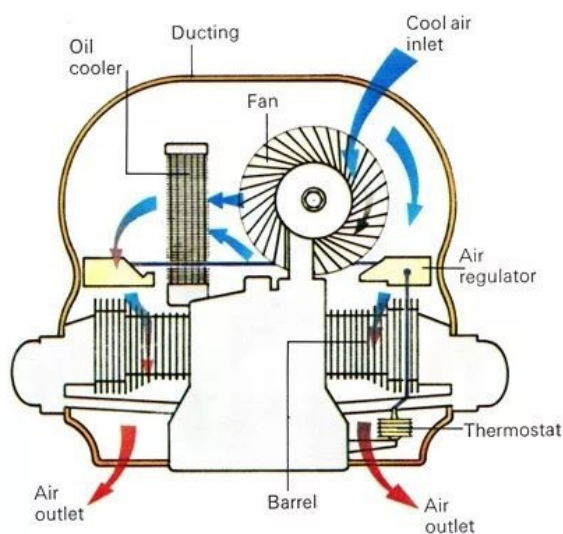
Figure 1.1.3: Principle of air-cooling system
