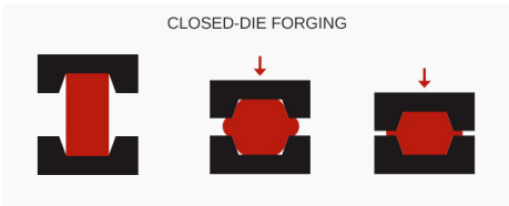
Figure. 4.16.5: Closed die forging
