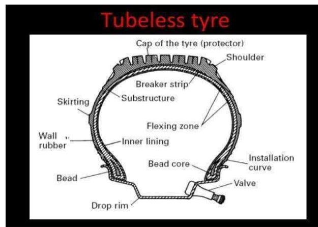
Figure 6.23.4: Features of a tyre and rim assembly
