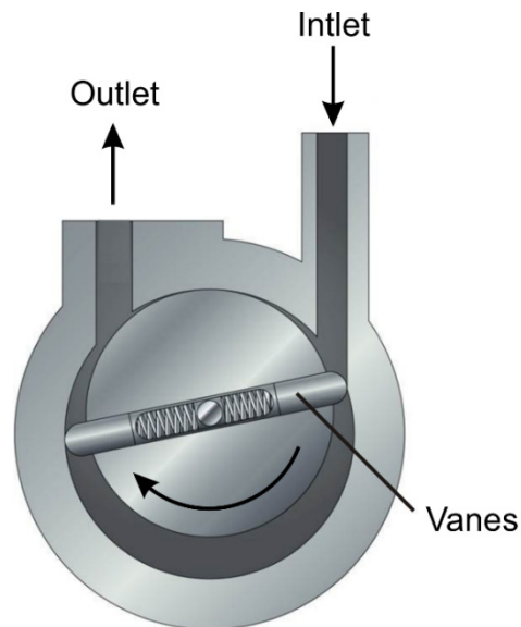
Figure. 3.9.6: Vane-type oil pump
