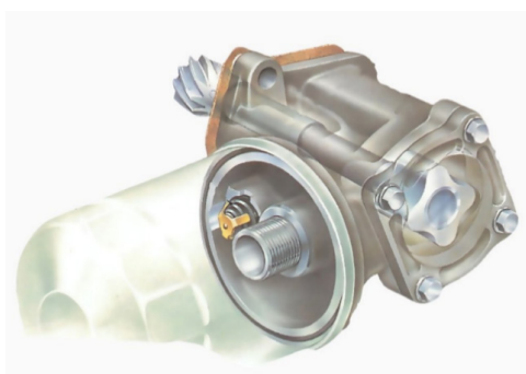
Figure. 2.7.6: An oil pump assembly
