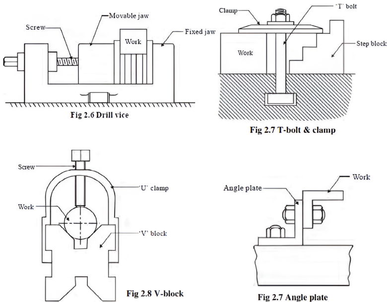
Figure 1.4.7: Devices used for holding the work in a drilling machine
