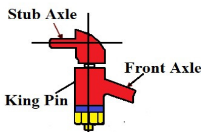
Figure 4.13.8: Reversed Lemoine stub axle
