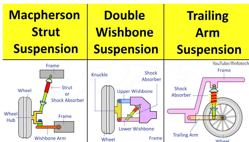
Figure 6.21.3: Types of Independent front suspension systems
