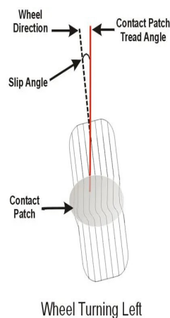
Figure. 4.15.15: Slip angle
