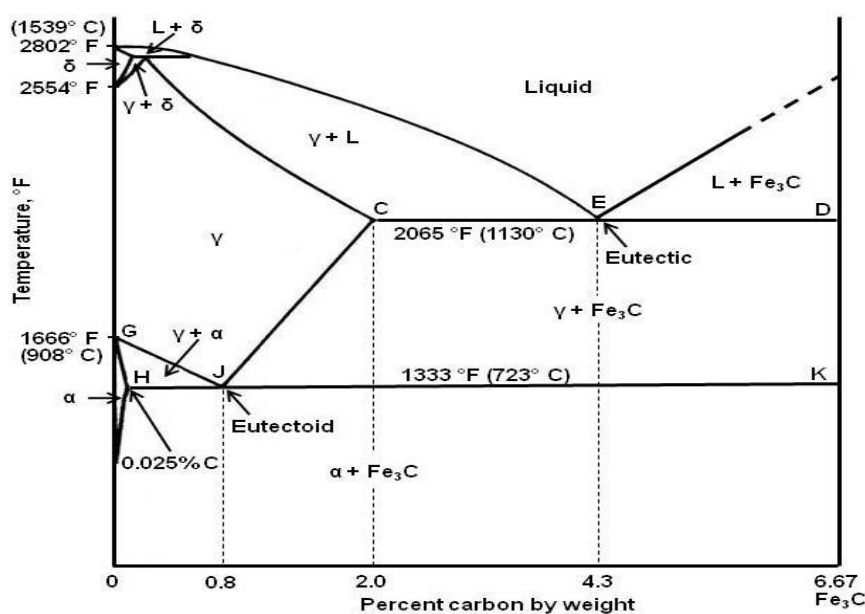
Figure 1.2.2: Iron-carbon equilibrium diagram.
