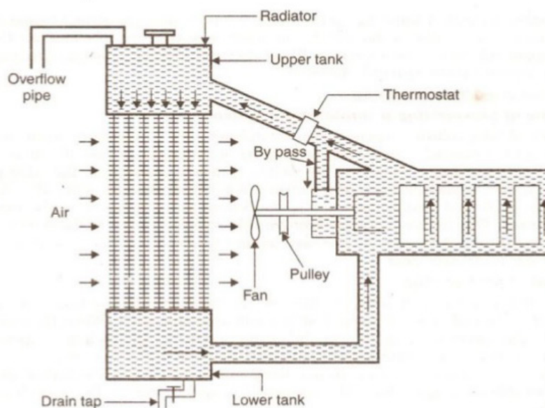
Figure 1.3.6: Thermosiphon water cooling system
