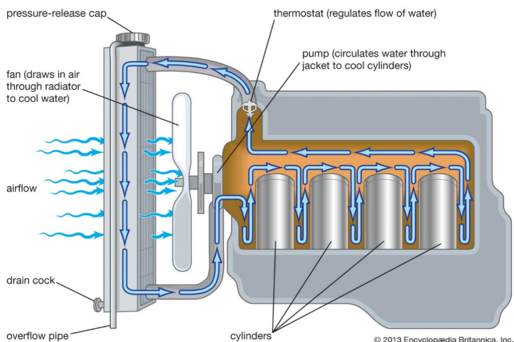
Figure. 2.5.3: Pressurised water-cooling system
