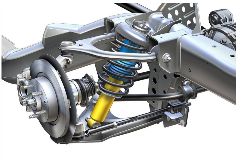
Figure 6.21.8: Multi-link suspension
