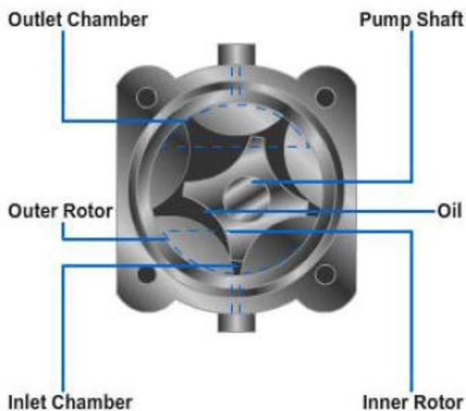
Figure. 3.9.5: Rotor oil pump
