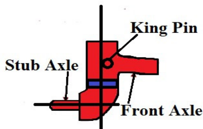
Figure. 4.13.7: Lemoine stub axle
