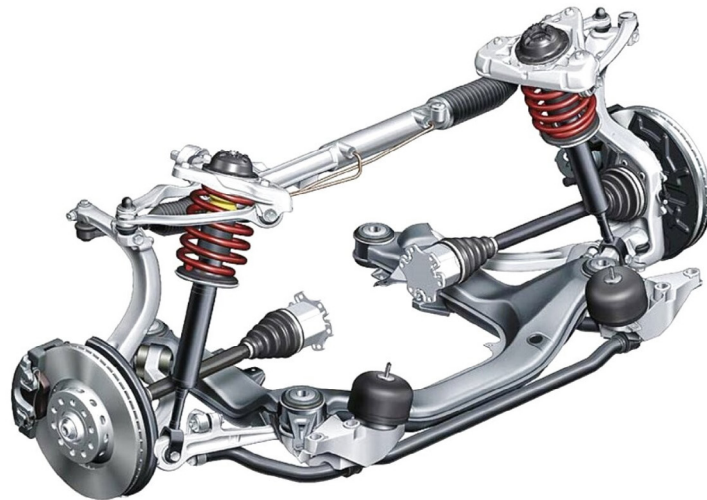
Figure 6.21.9: double wishbone suspension
