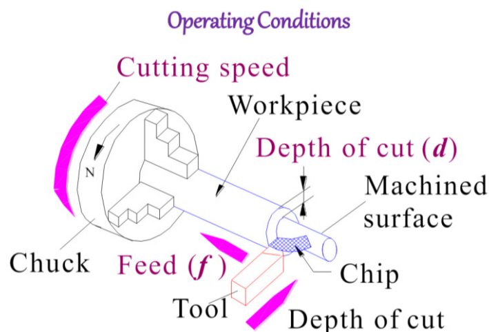
Figure. 2.6.2: Parallel turning indicating operating conditions on the lathe machine
