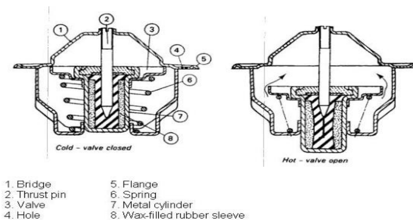
Figure. 2.5.2: A wax-type thermostat in closed and open positions
