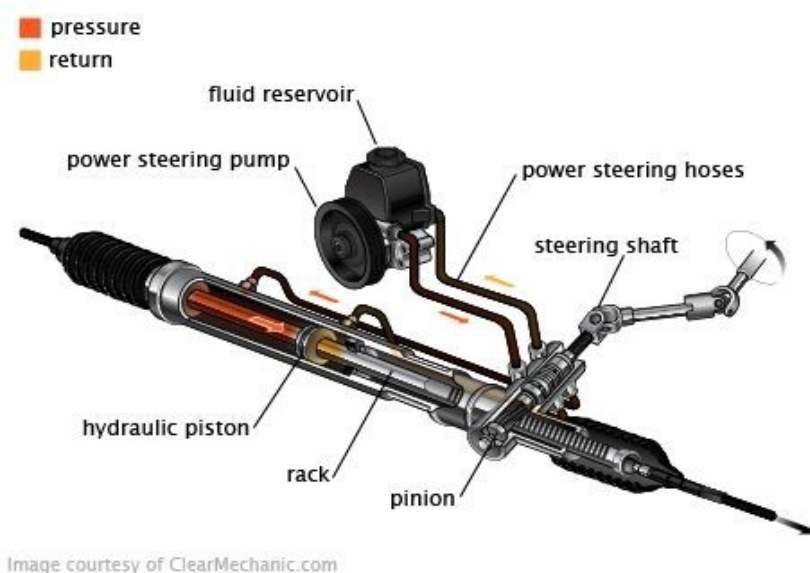
Figure. 4.15.2: A power-assisted steering mechanism
