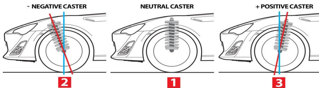
Figure. 4.15.8: Castor angles
