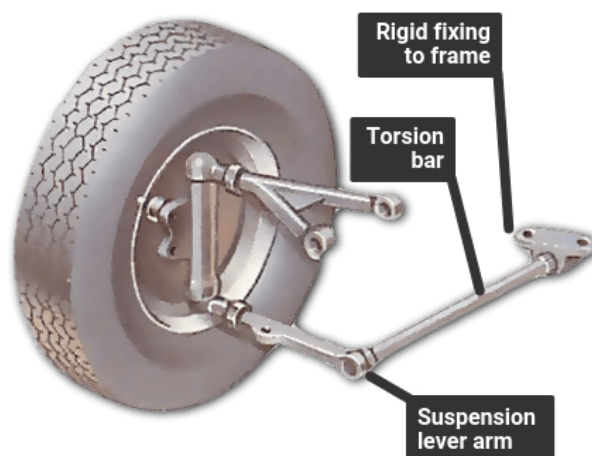
Figure. 5.19.6: Torsion bar in suspension system
