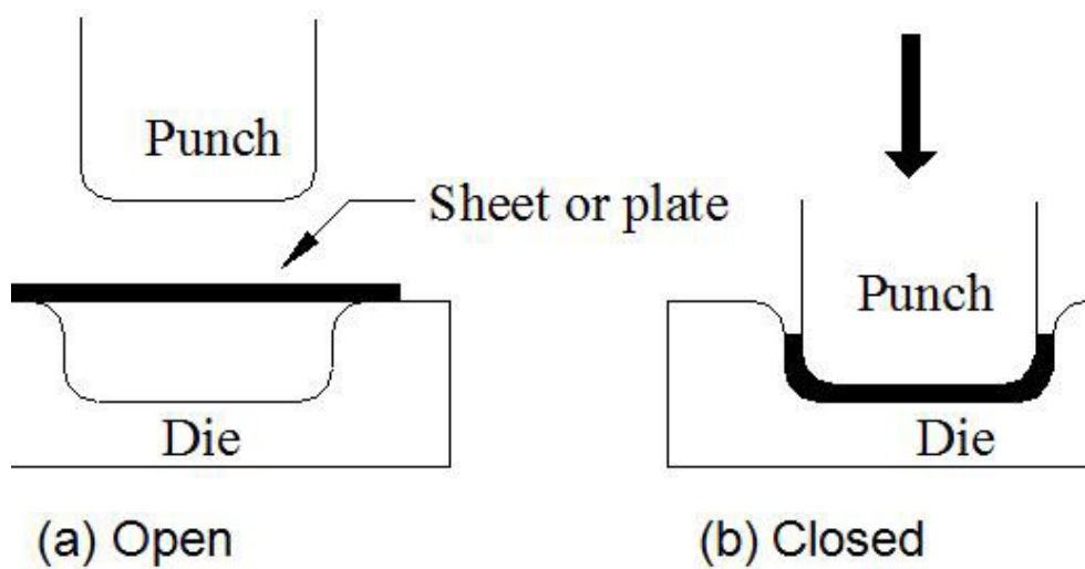
Figure 5.18.1: Punches and Dies
