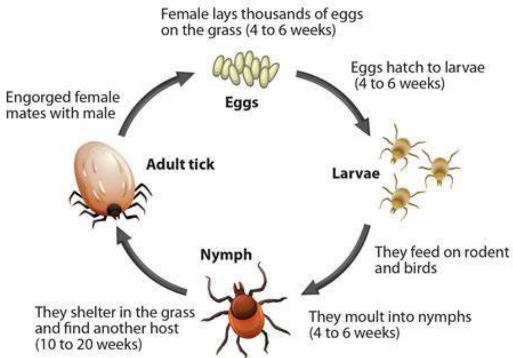
Figure 6.4: Developmental stages of a tick species
