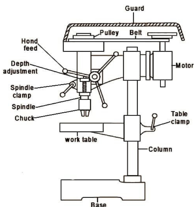
Figure 4.6: Parts of a drilling machine
