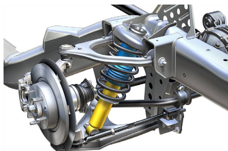
Figure 21.8: Multi-link suspension
