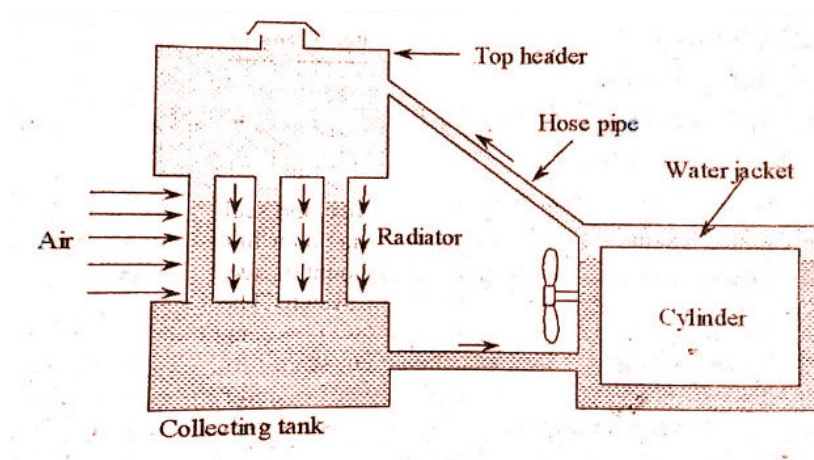
Figure 3.6: Thermosiphon water cooling system
