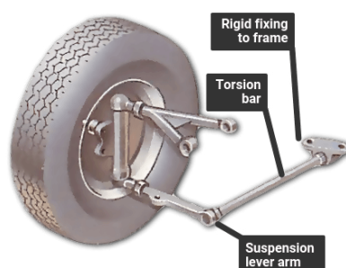
Figure 19.6: Torsion bar in suspension system
