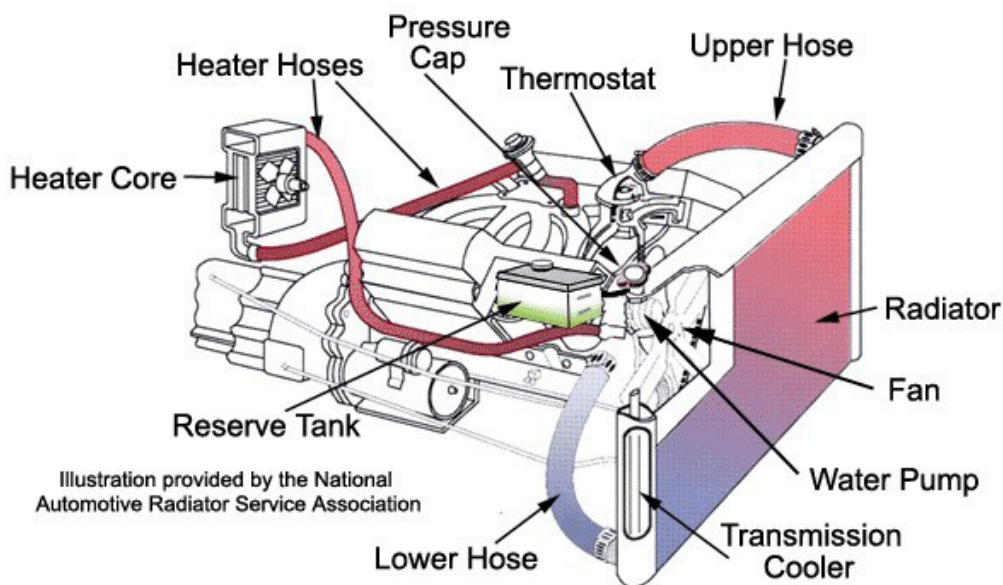
Figure 3.8: Pump-assisted water-cooling system
