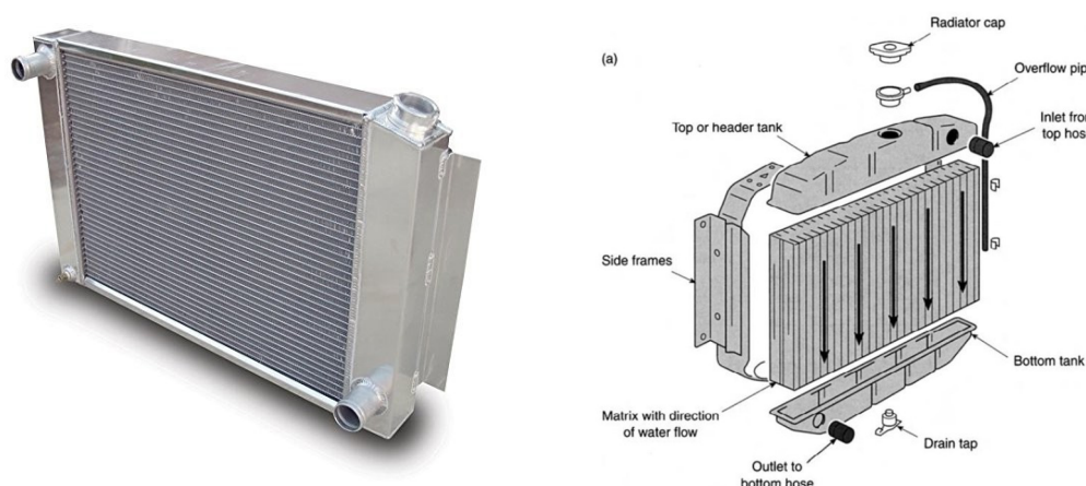
Figure 3.4: Radiator
