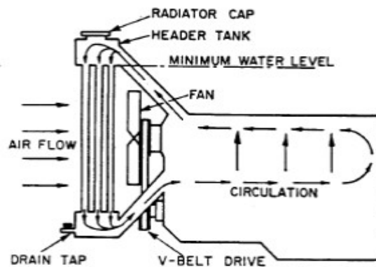
Thermo-syphon system.
