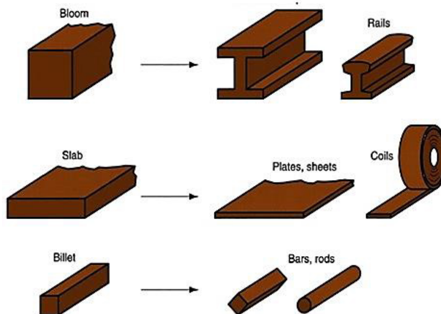
Figure 16.8: Some of the steel products made in a rolling mill.
