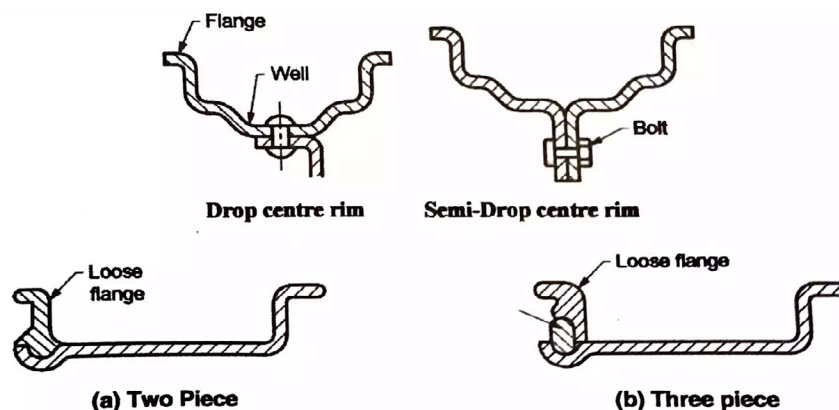
Figure 23.6: Flat-base rims
