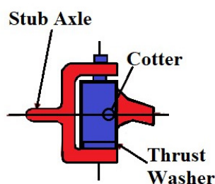
Figure 13.6: Reversed Elliot stub axle
