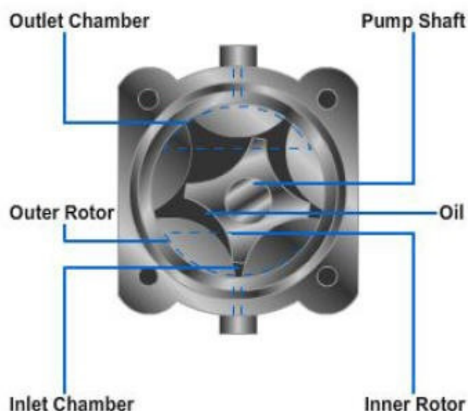
Figure 9.5: Rotor oil pump
