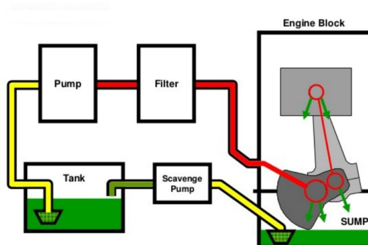
Figure 7.4: Dry sump lubrication system.
