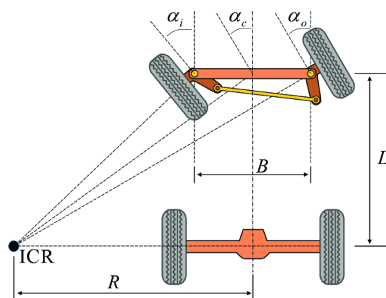
Figure 15.13: Ackermann steering geometry
