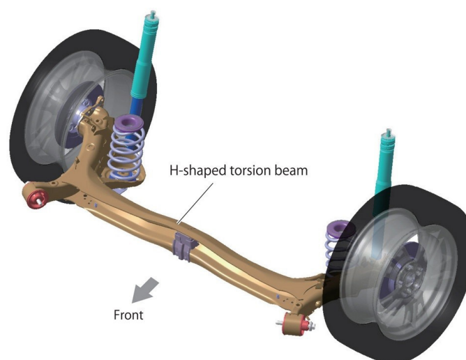
Figure 17.5: Dependent/axle beam suspension system
