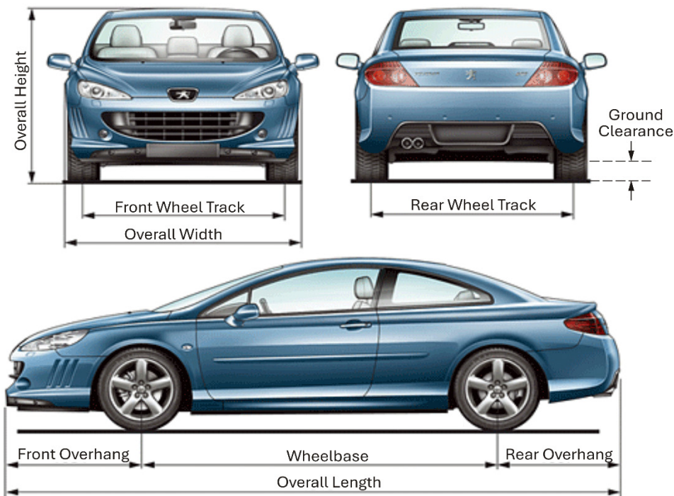
Figure 13.9: Vehicle dimensions
