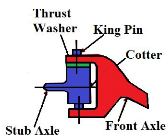
Figure 13.5: Elliot stub axle
