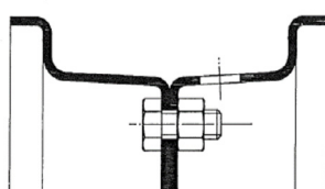
Figure 23.8: A divided rim
