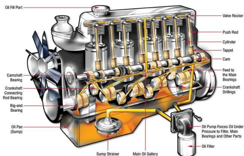
Figure 7.2: Oil distribution channels in the engine.
