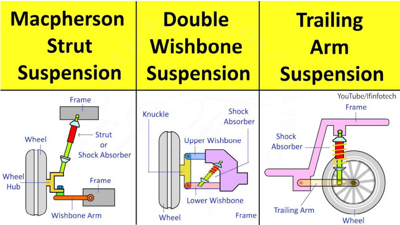
Figure 21.3: Types of Independent front suspension systems
