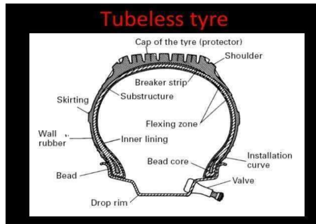
Figure 23.4: Features of a tyre and rim assembly
