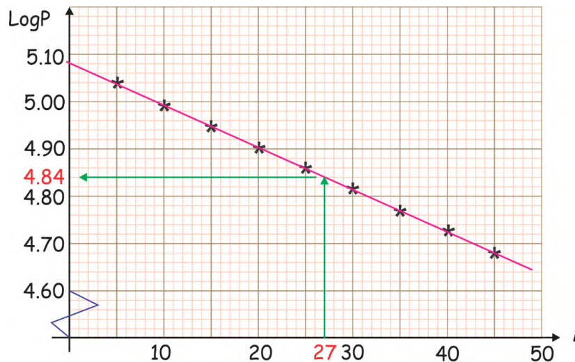
Figure 8.7: Graph of the relation P = ab^t ,
