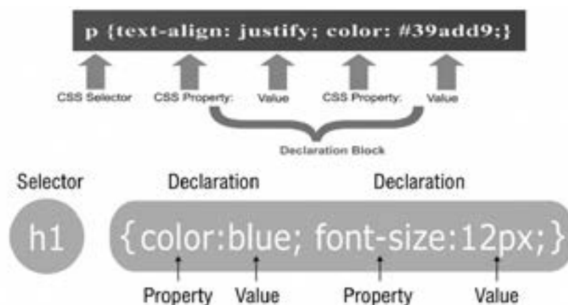
Figure 6.3: The syntax rule
