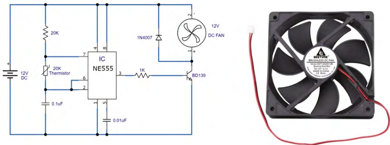
Figure 18: A picture of the electrical circuit of a temperature-controlled fan
