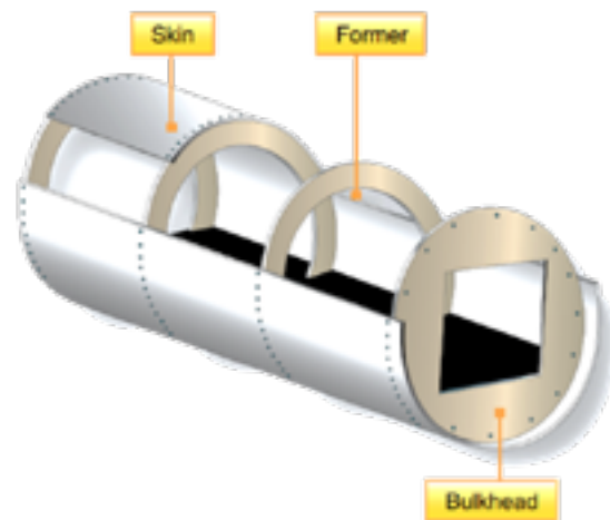
Figure 1.10: Monocoque fuselage
