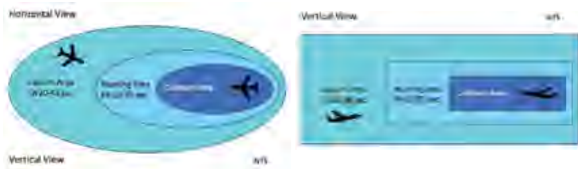
Figure 3.16: TCAS protection volume
