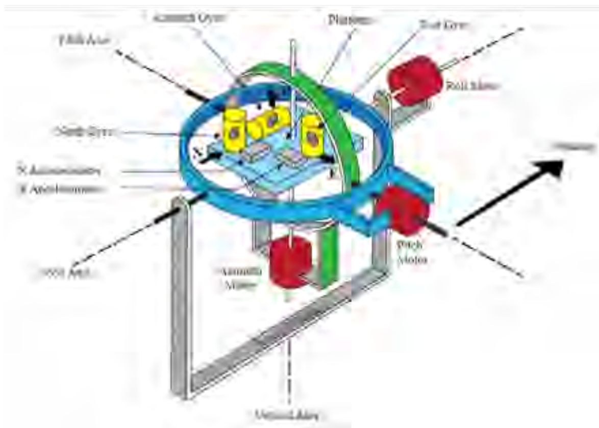
Figure 3.5: Stable platform INS
