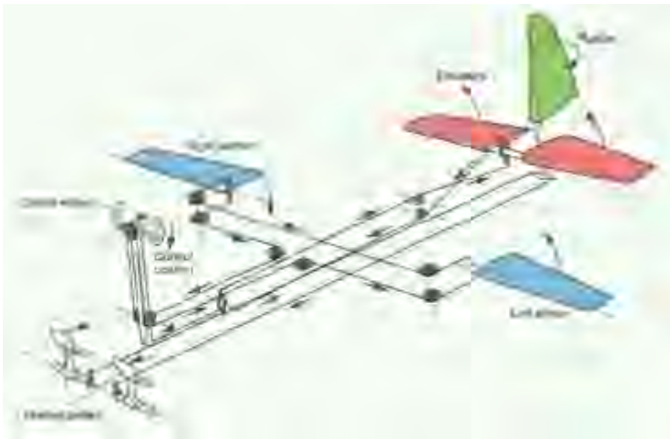
Figure 2.14: Mechanical flight control system
