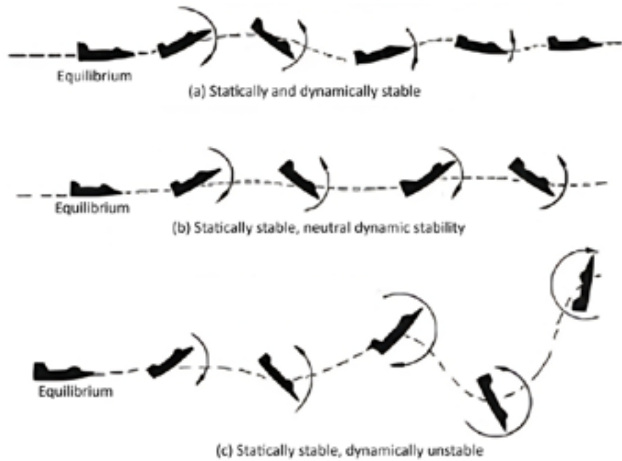
Figure 2.17: Aircraft stability
