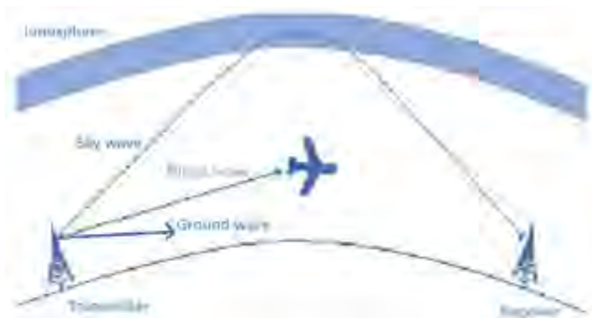
Figure 3.2: HF communication pathways
