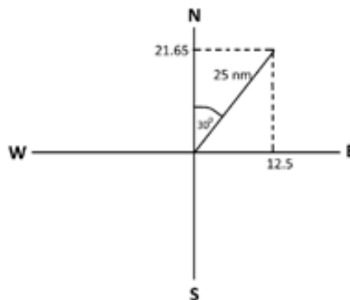
Figure 3.4: Dead reckoning calculation
