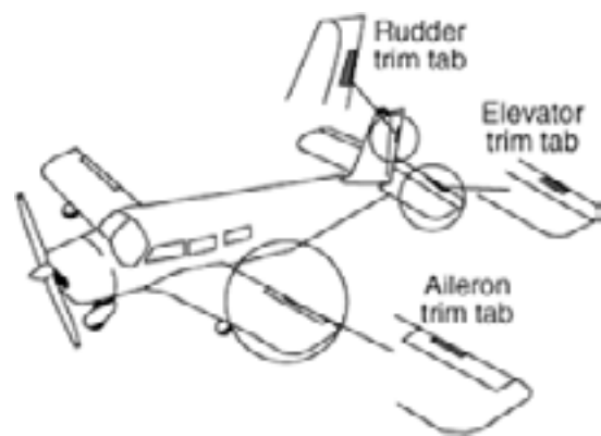
Figure 2.7: Trim tabs
