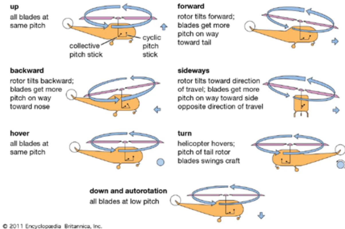
Figure 2.9: Effects of helicopter control inputs
