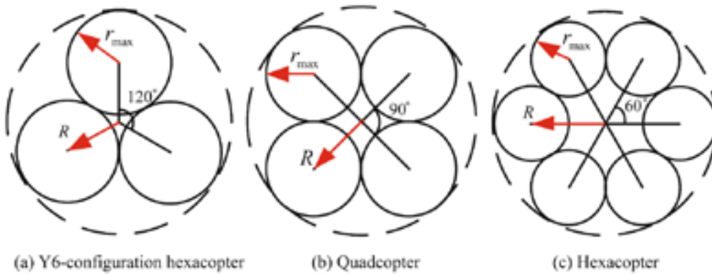
Figure 5.5: Multicopter arm length
