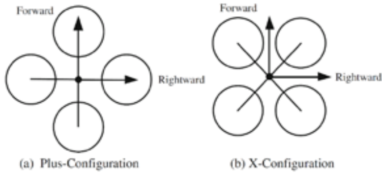
Figure 5.4: Plus and X quadcopter configurations
