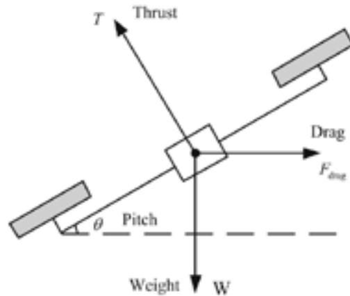
Figure 5.3: Multirotor UAV in forward flight
