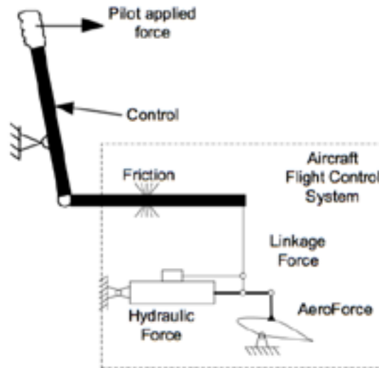
Figure2.15: Hydraulic flight control system
