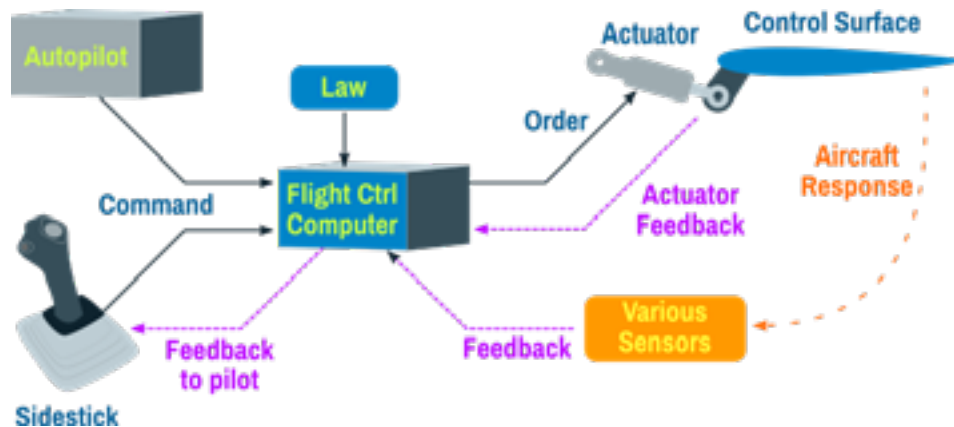
Figure 2.16: Fly-by-wire control system
