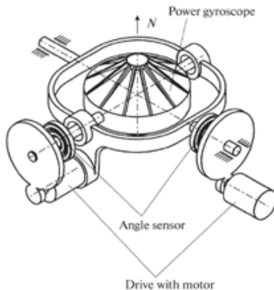
Figure 2.12: Control moment gyroscope
