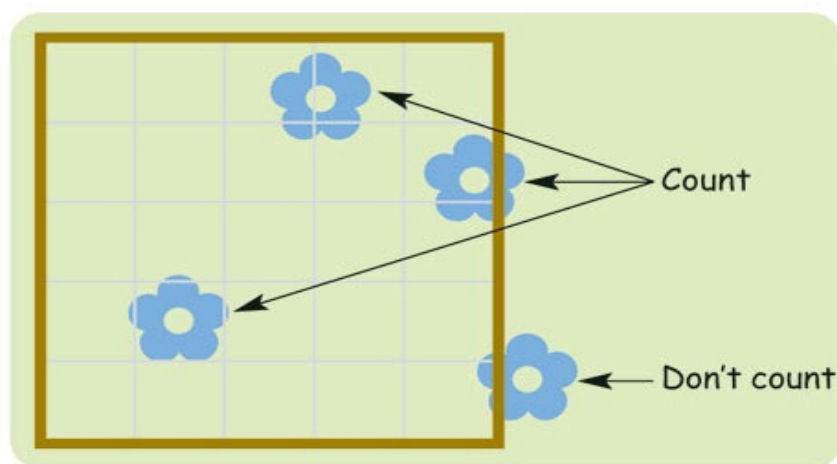
Figure 3.23: Using a quadrat to sample
