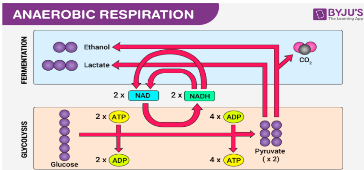
Figure 4.7: Pathway for anaerobic respiration (fermentation) in plants and animals.
