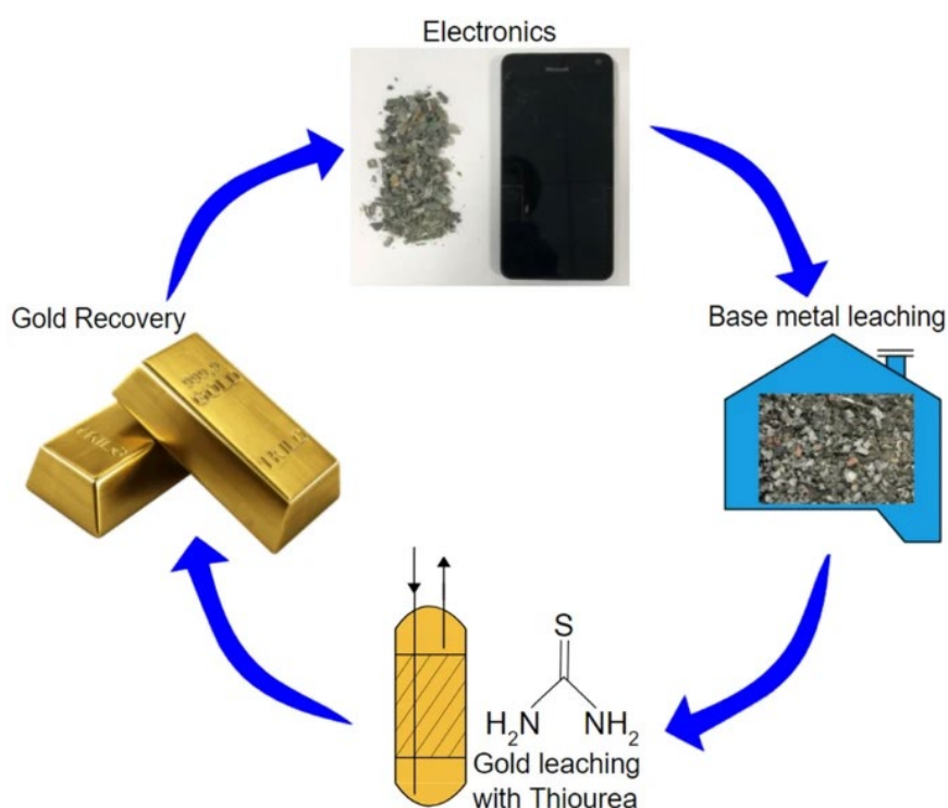
Figure 1.11: A chart showing gold extraction from electronic waste by bioleaching
