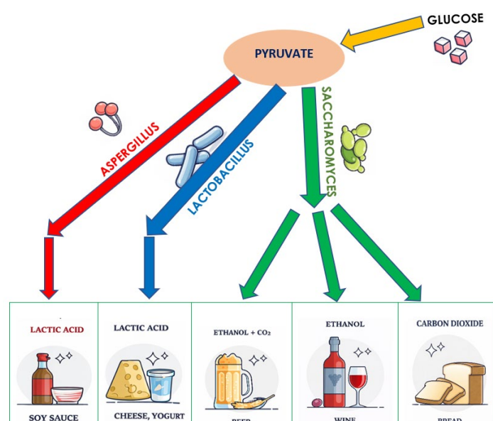
Figure 1.1: Types of microbial fermentation from pyruvate and their associated food products
