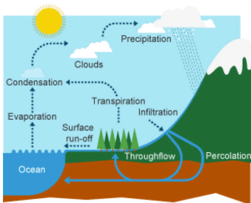
Figure 3.13: Water cycle
