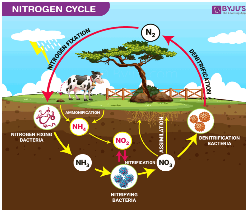
Figure 3.12: Nitrogen cycle
