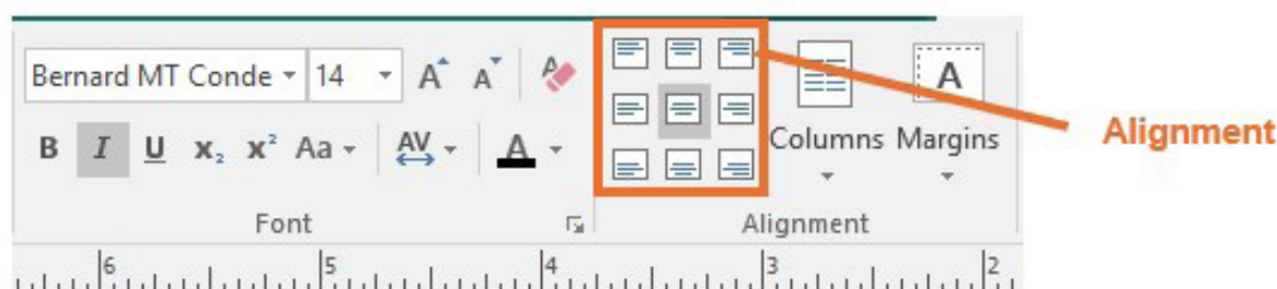
Figure 1.19: Alignment Controls
