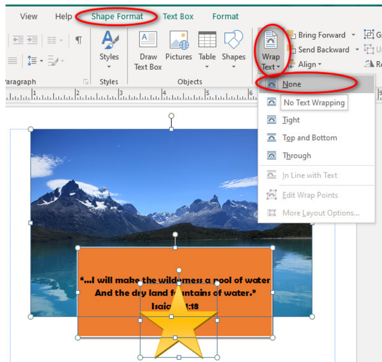
Figure 1.38: Layering
