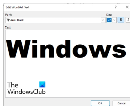
Figure 1.33: Formatting WordArt
