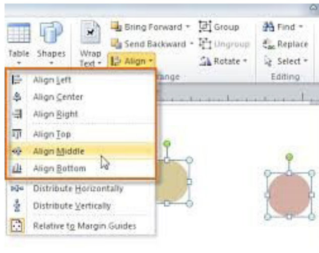
Figure 1.43: Alignment Guides
