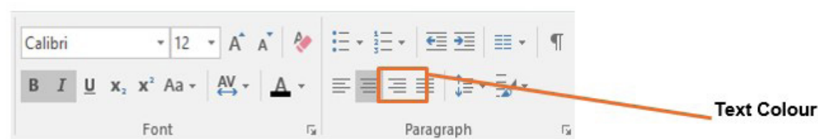
Figure 1.23: Text Colour
