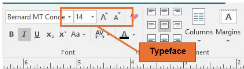
Figure 1.16: Typeface
