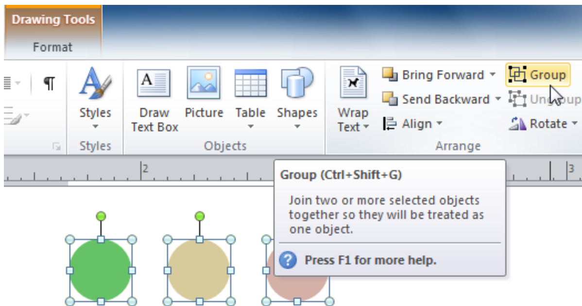
Figure 1.41: Grouping Objects
