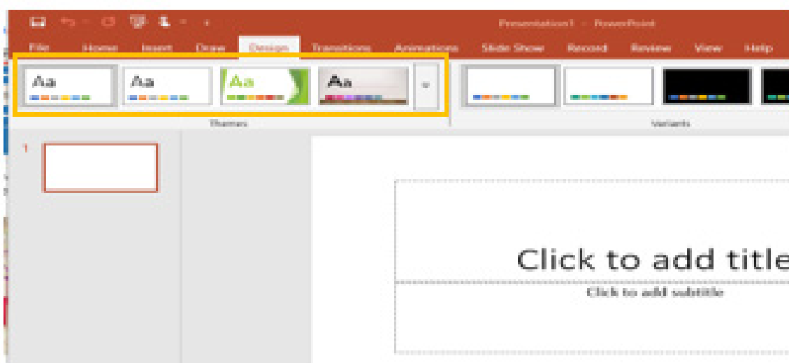
Figure 1.10: Presentation Themes
