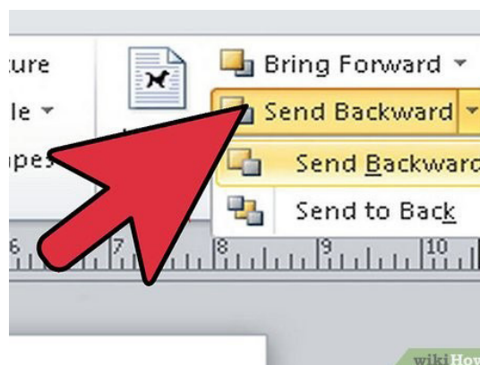
Figure 1.39: Layering Tools
