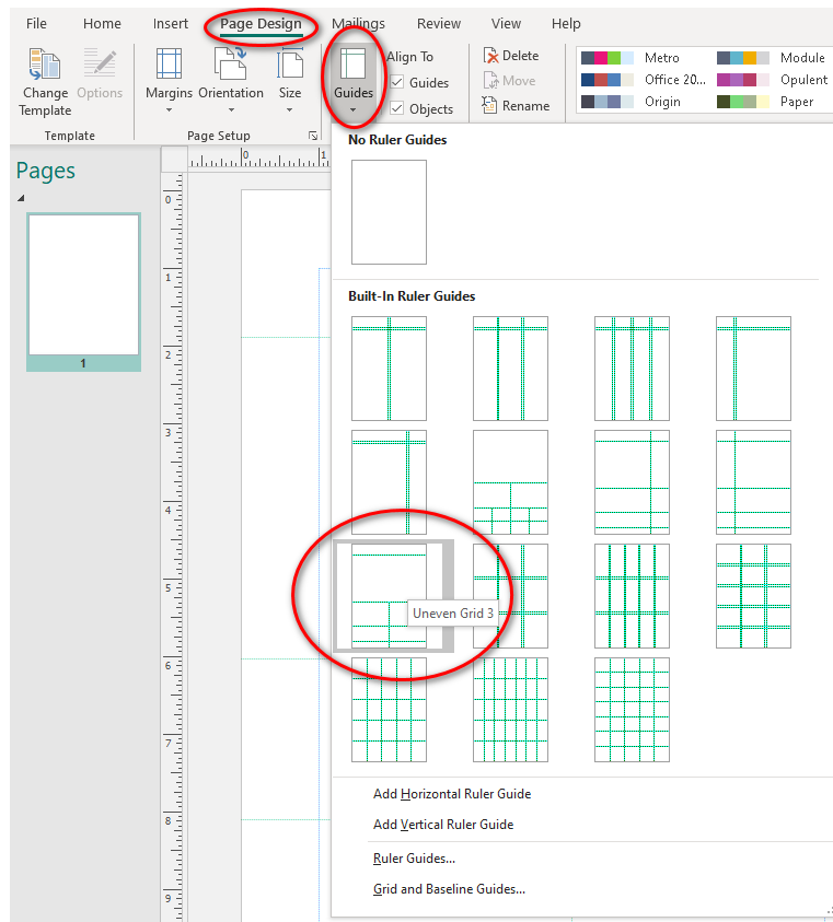
Figure 1.44: Smart Guides
