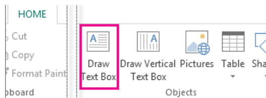
Figure 1.29: Text Box
