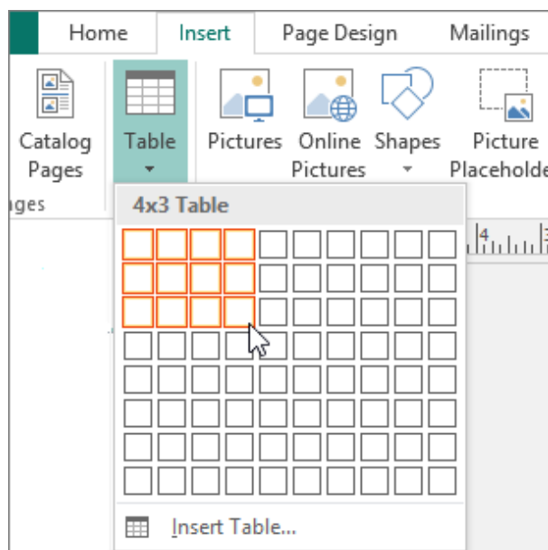
Figure 1.30: Inserting Tables
