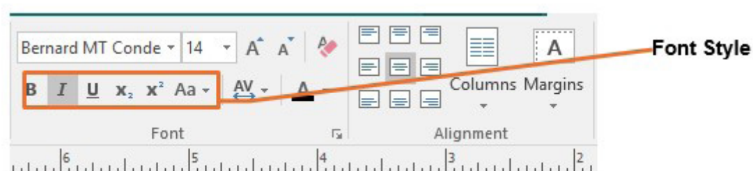
Figure 1.18: Font Style
