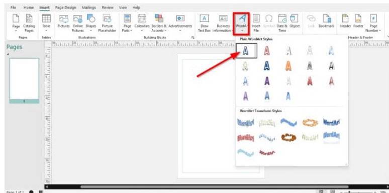
Figure 1.32: Inserting WordArt
