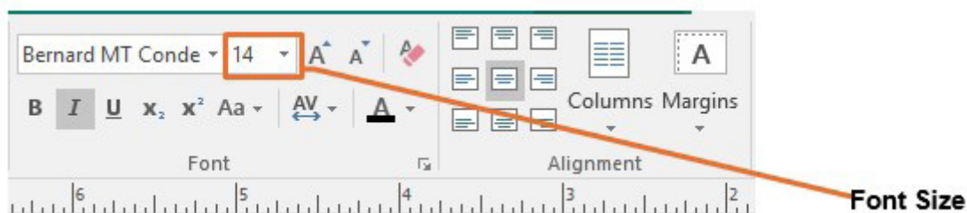
Figure 1.17: Font Size
