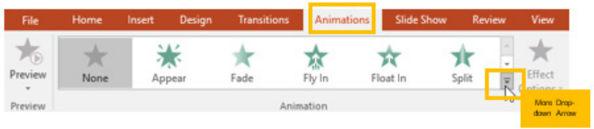
Figure 1.5: Animation Tab
