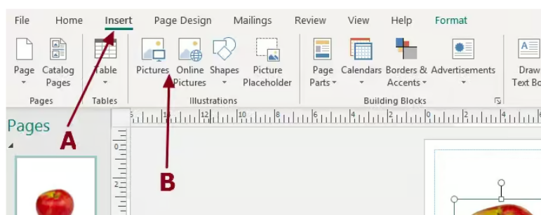
Figure 1.31: Inserting Picture
