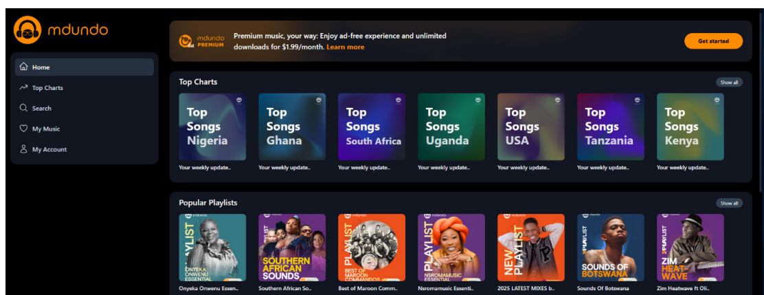
Figure 4.12: Audio Platform
