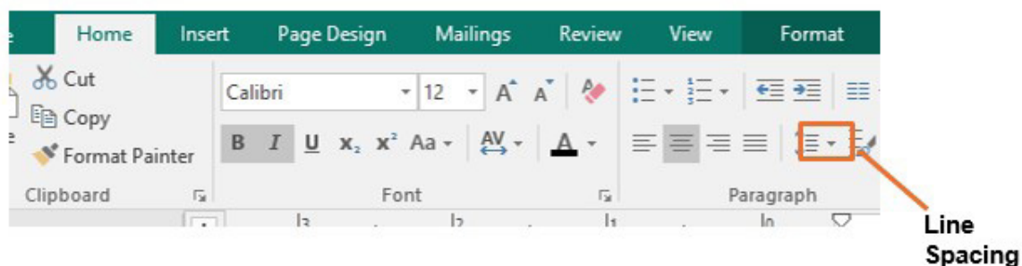
Figure 1.20: Line Spacing
