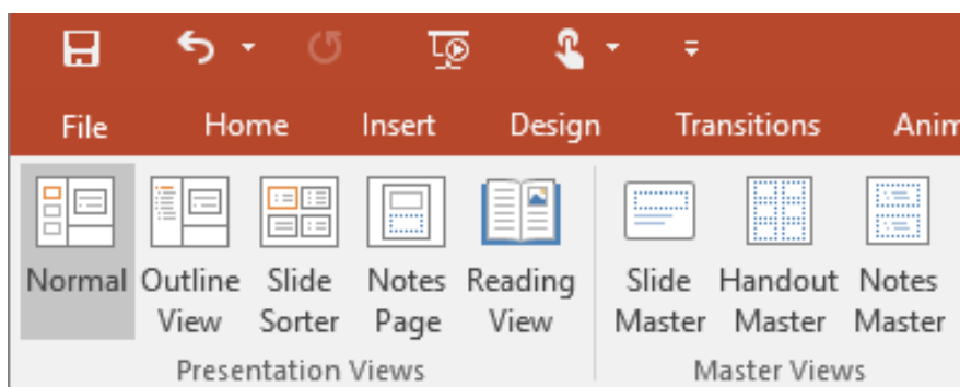
Figure 1.9: Presentation views
