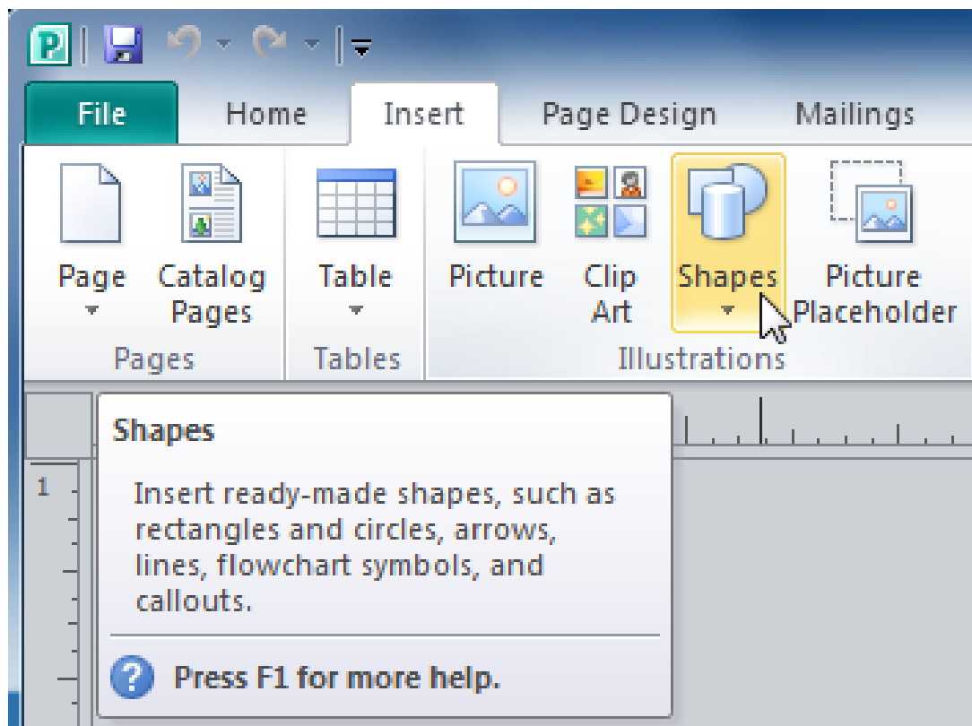
Figure 1.40: Adding Shapes
