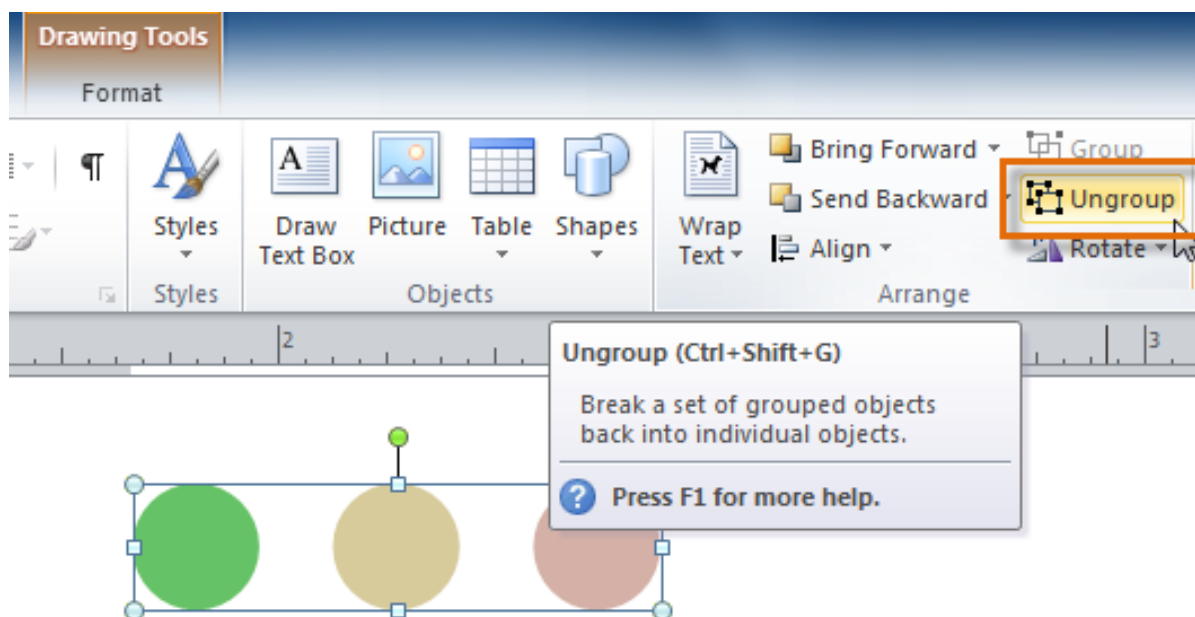
Figure 1.42: Ungrouping Objects
