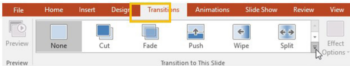
Figure 1.7: Transition Tab
